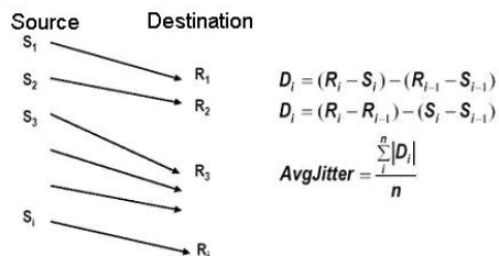
Figure 1: Jitter formula
